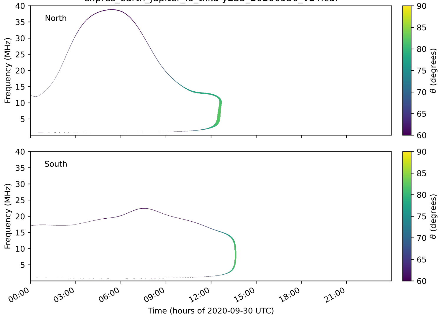
expres_earth_jupiter_io_txka-y235_20200930_v14.cdf
