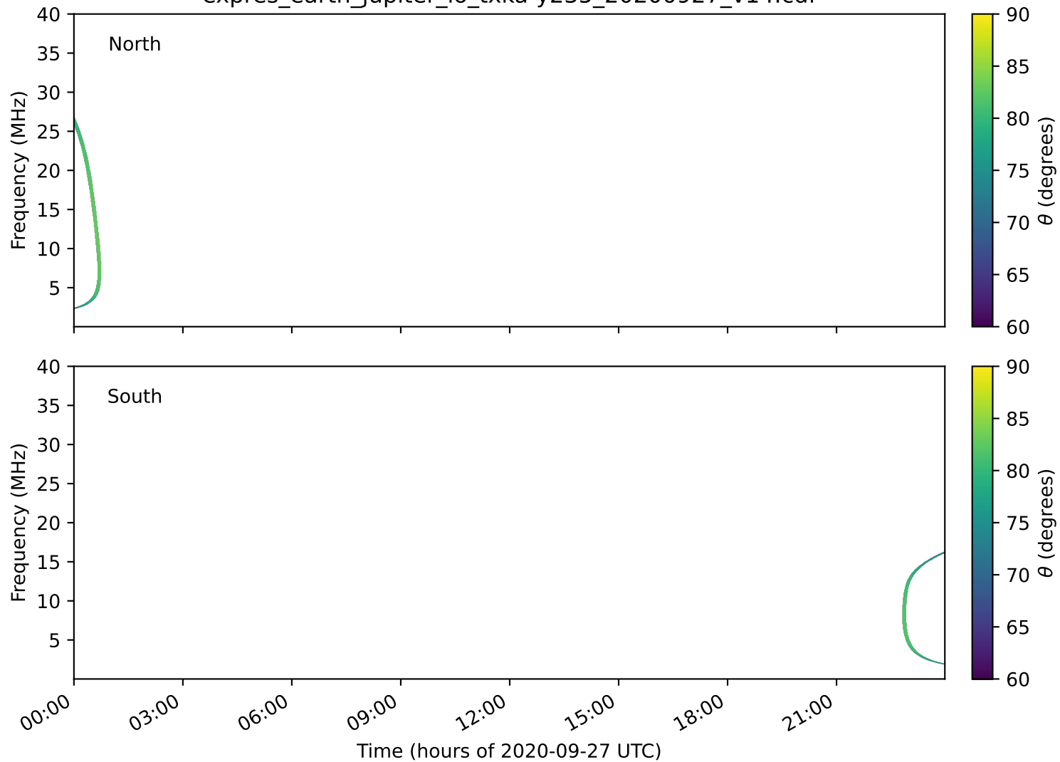
expres_earth_jupiter_io_txka-y235_20200927_v14.cdf
