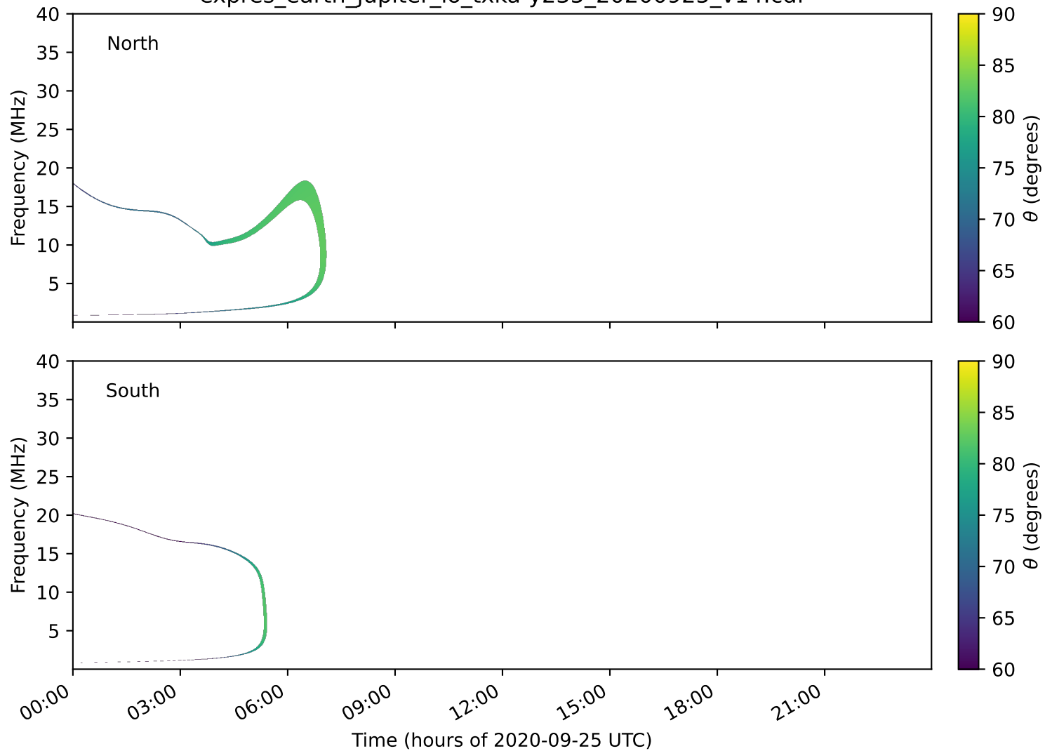
expres_earth_jupiter_io_txka-y235_20200925_v14.cdf
