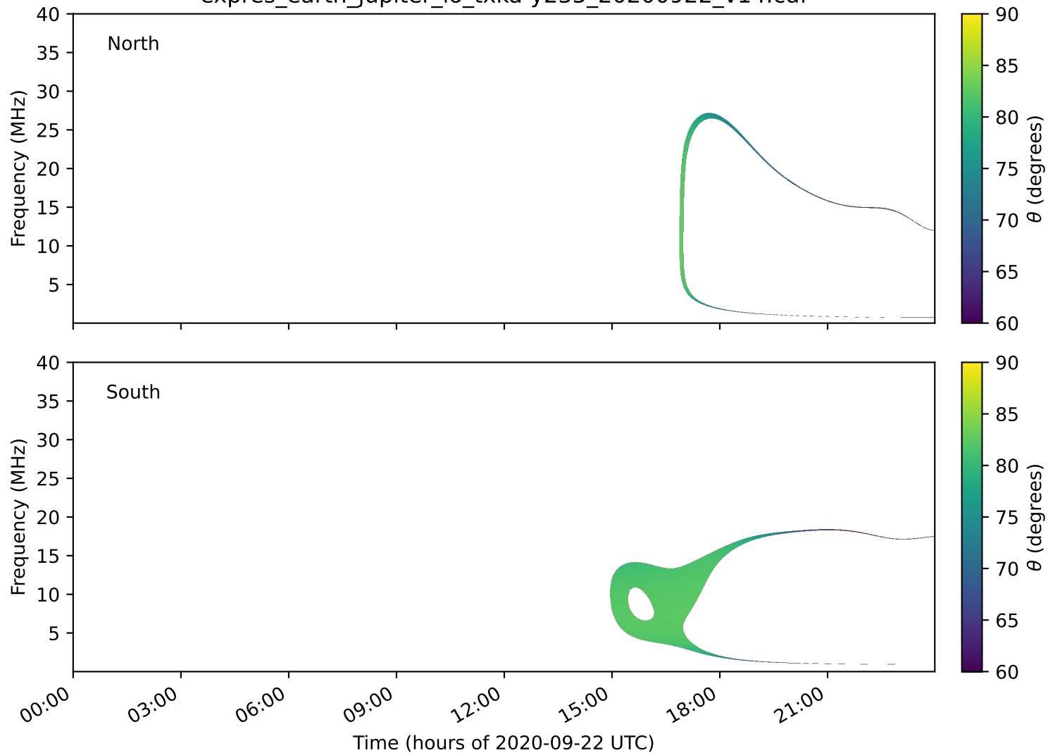
expres_earth_jupiter_io_txka-y235_20200922_v14.cdf
