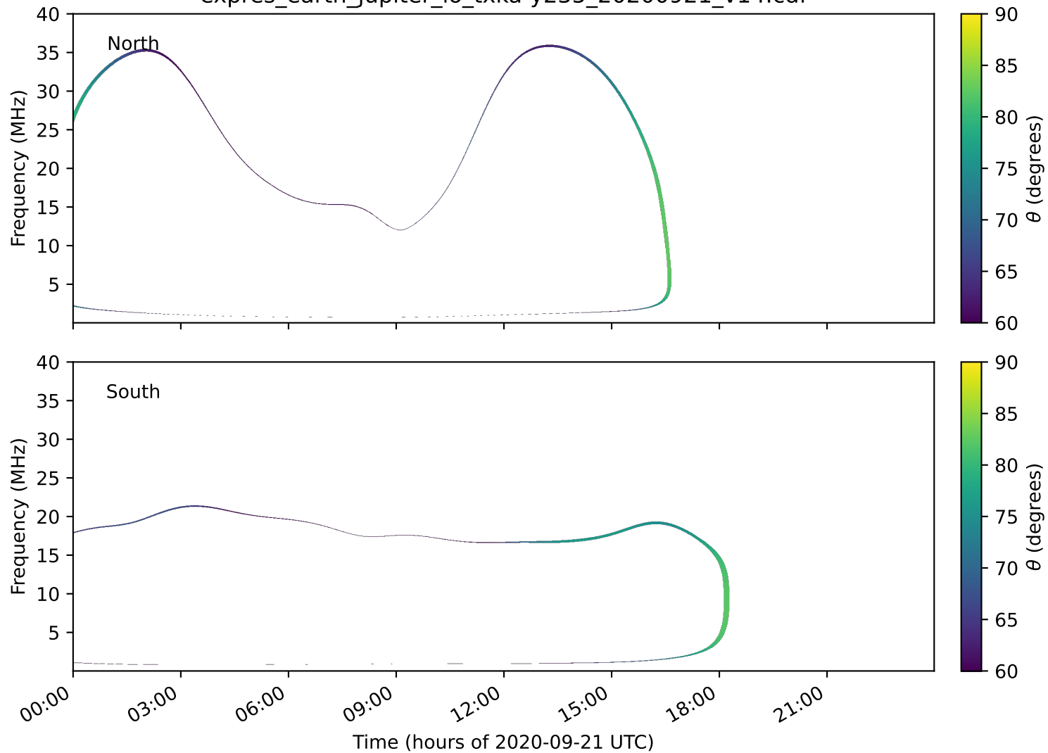
expres_earth_jupiter_io_txka-y235_20200921_v14.cdf
