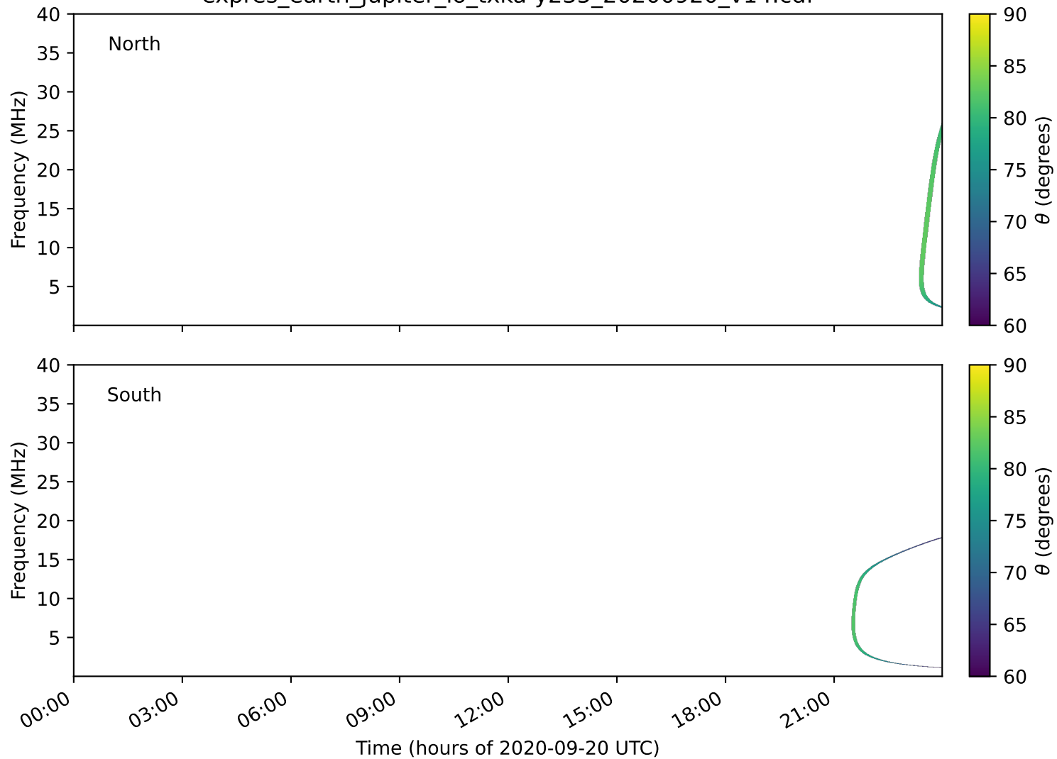
expres_earth_jupiter_io_txka-y235_20200920_v14.cdf
