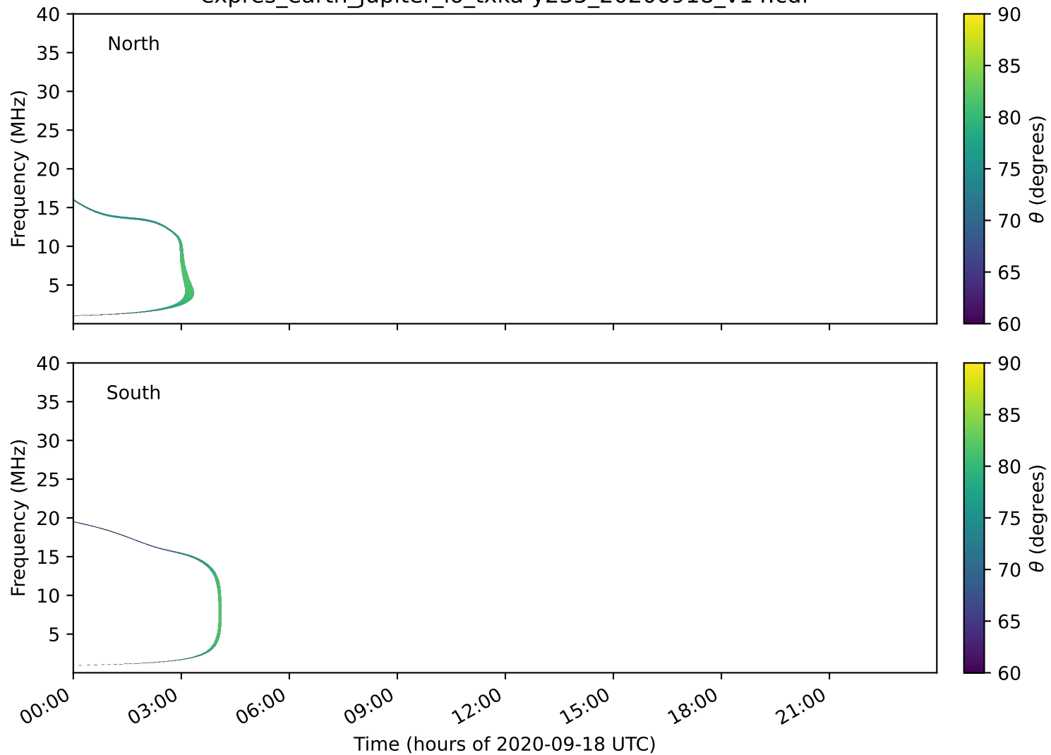
expres_earth_jupiter_io_txka-y235_20200918_v14.cdf
