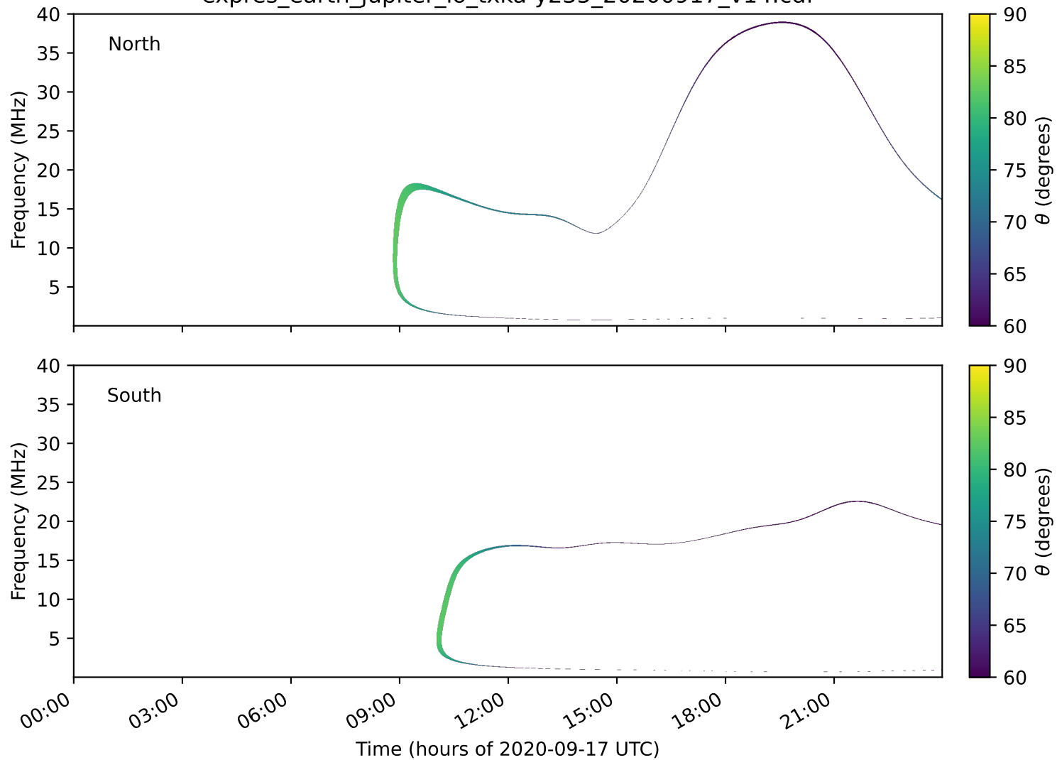
expres_earth_jupiter_io_txka-y235_20200917_v14.cdf
