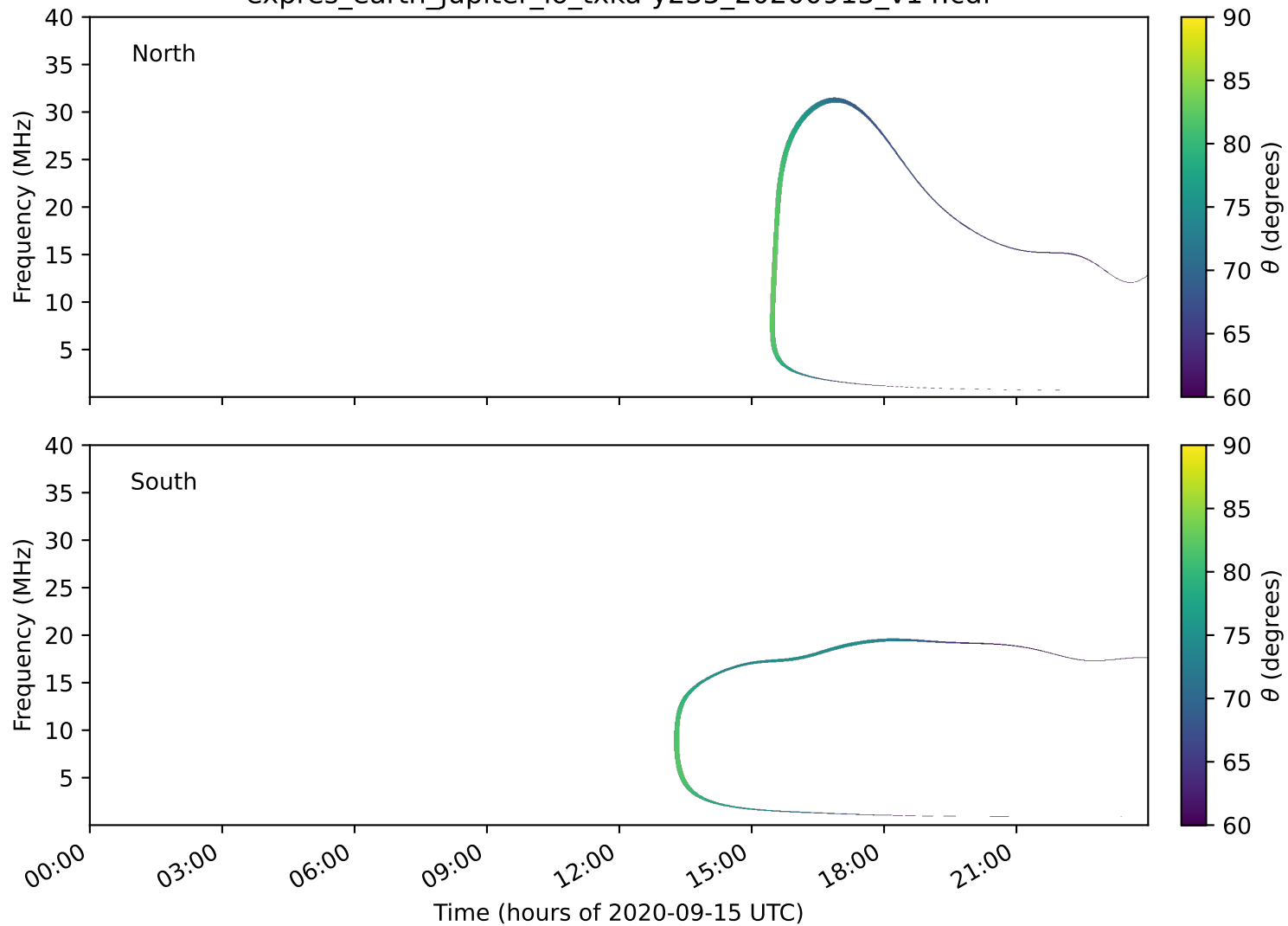
expres_earth_jupiter_io_txka-y235_20200915_v14.cdf
