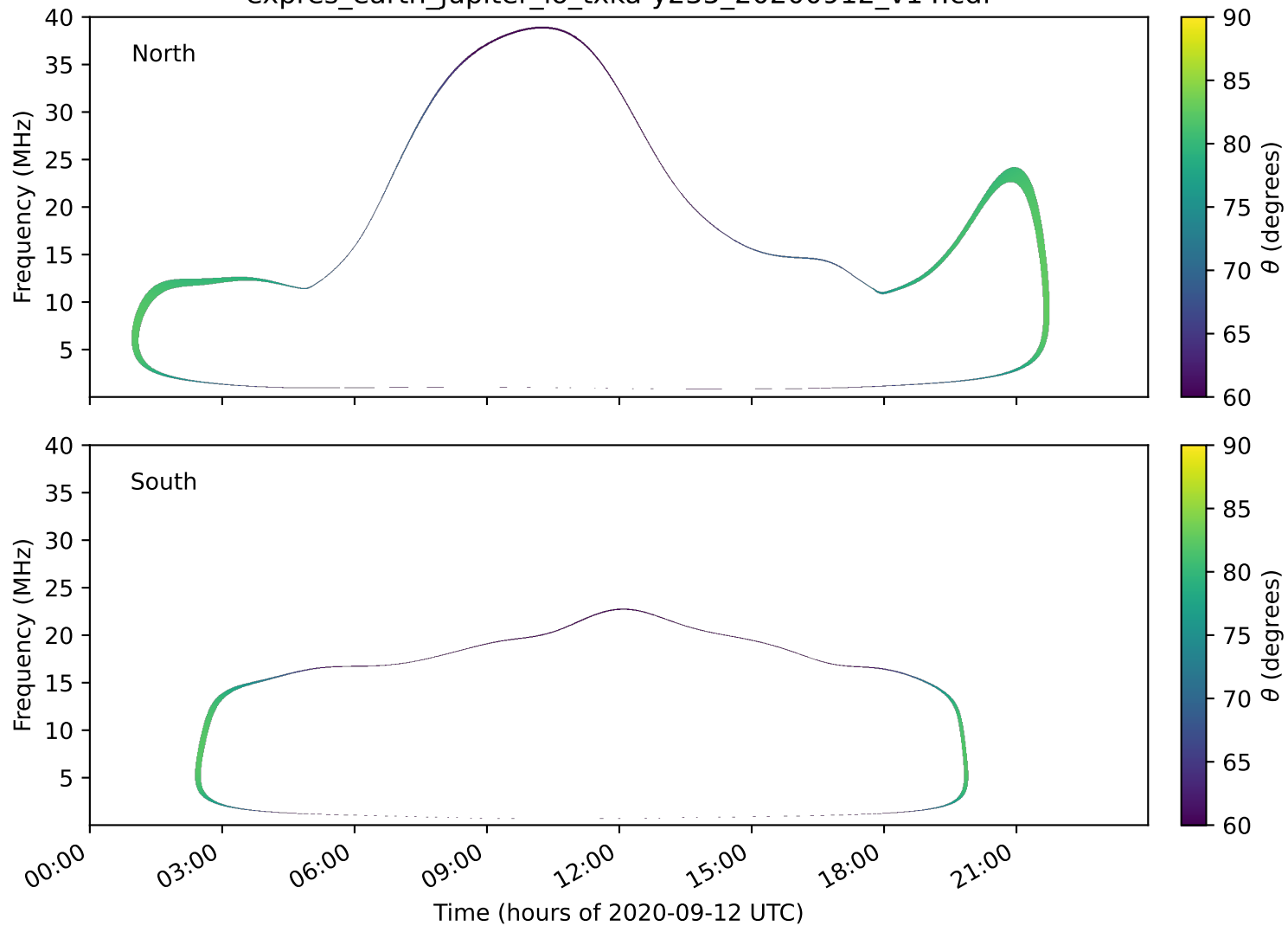
expres_earth_jupiter_io_txka-y235_20200912_v14.cdf
