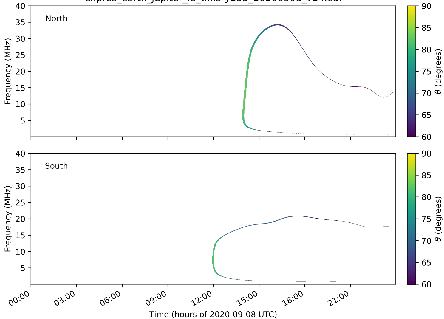
expres_earth_jupiter_io_txka-y235_20200908_v14.cdf
