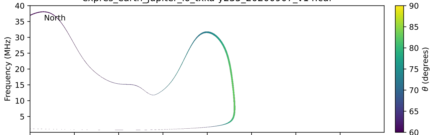
expres_earth_jupiter_io_txka-y235_20200907_v14.cdf
