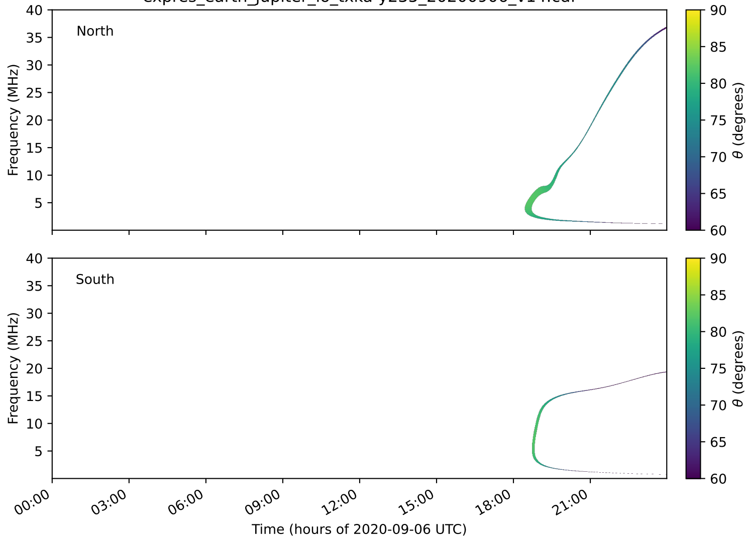
expres_earth_jupiter_io_txka-y235_20200906_v14.cdf
