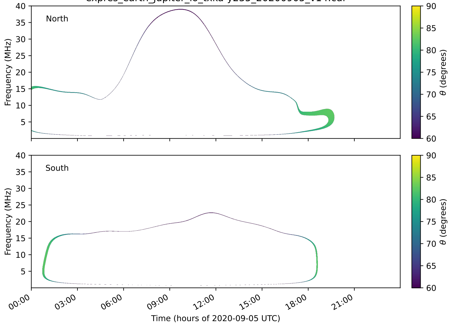
expres_earth_jupiter_io_txka-y235_20200905_v14.cdf
