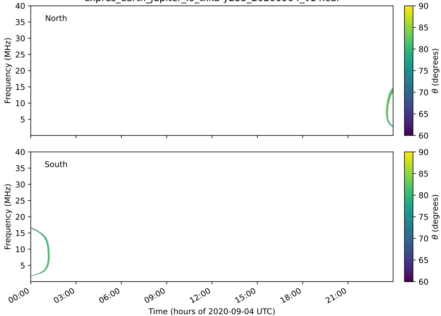
expres_earth_jupiter_io_txka-y235_20200904_v14.cdf
