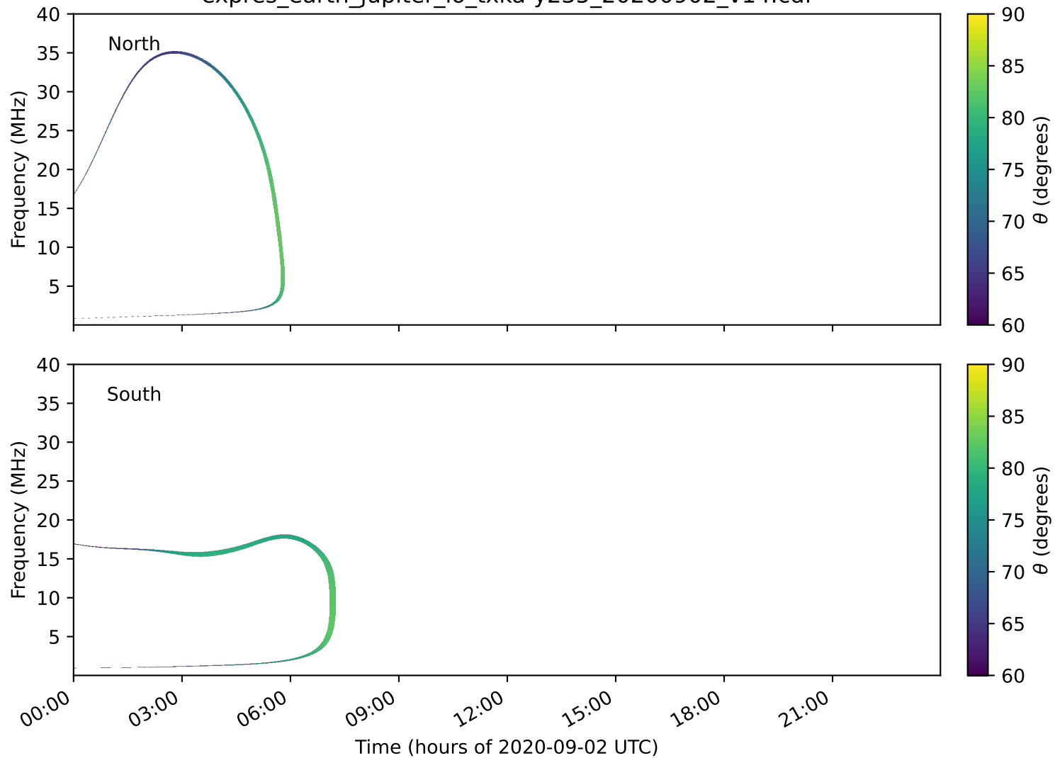
expres_earth_jupiter_io_txka-y235_20200902_v14.cdf
