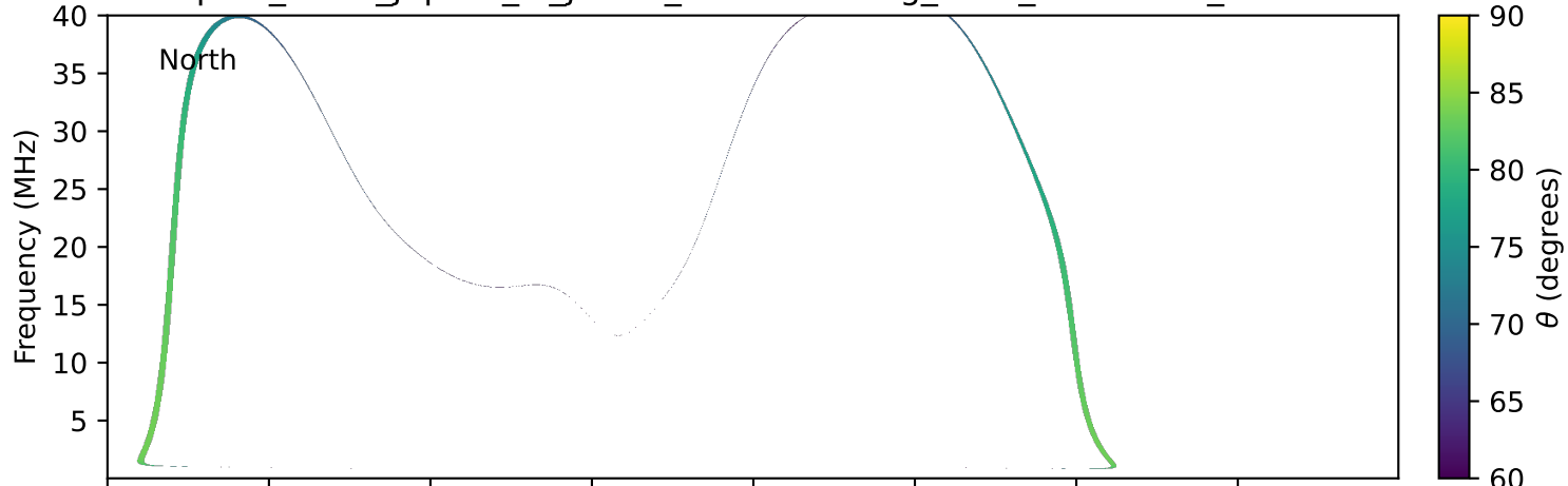
expres_earth_jupiter_io_jrm33_lossc-wid1deg_3kev_20200928_v11.cdf
