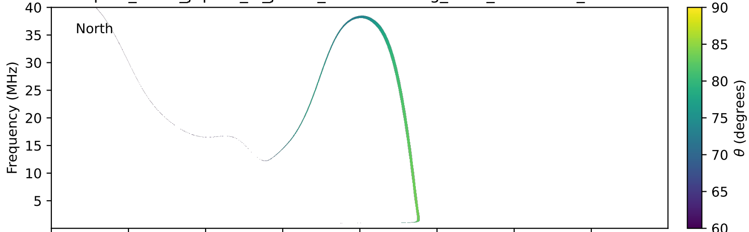
expres_earth_jupiter_io_jrm33_lossc-wid1deg_3kev_20200907_v11.cdf
