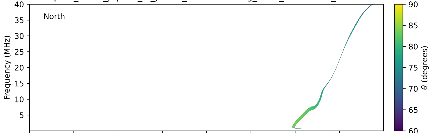
expres_earth_jupiter_io_jrm33_lossc-wid1deg_3kev_20200906_v11.cdf
