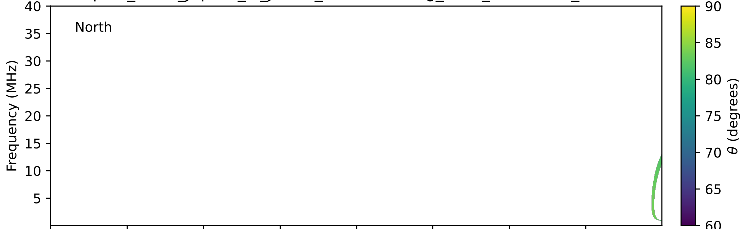
expres_earth_jupiter_io_jrm33_lossc-wid1deg_3kev_20200904_v11.cdf
