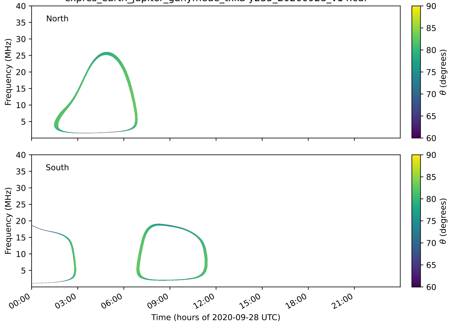
expres_earth_jupiter_ganymede_txka-y235_20200928_v14.cdf
