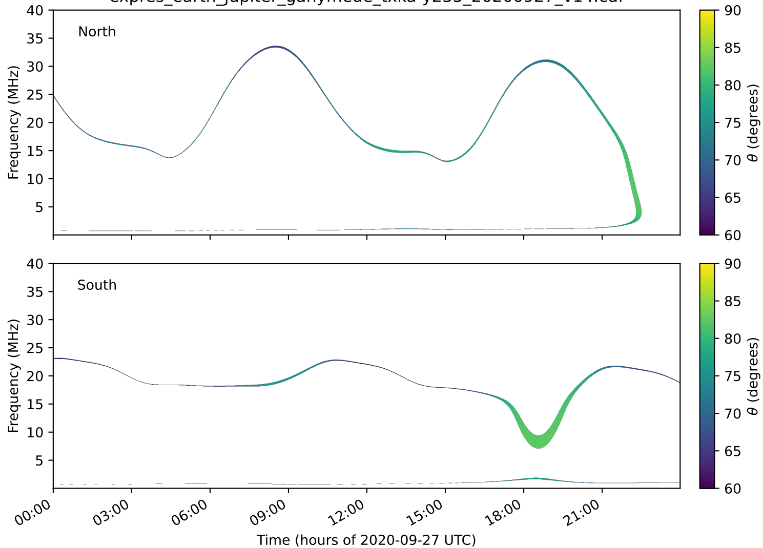
expres_earth_jupiter_ganymede_txka-y235_20200927_v14.cdf
