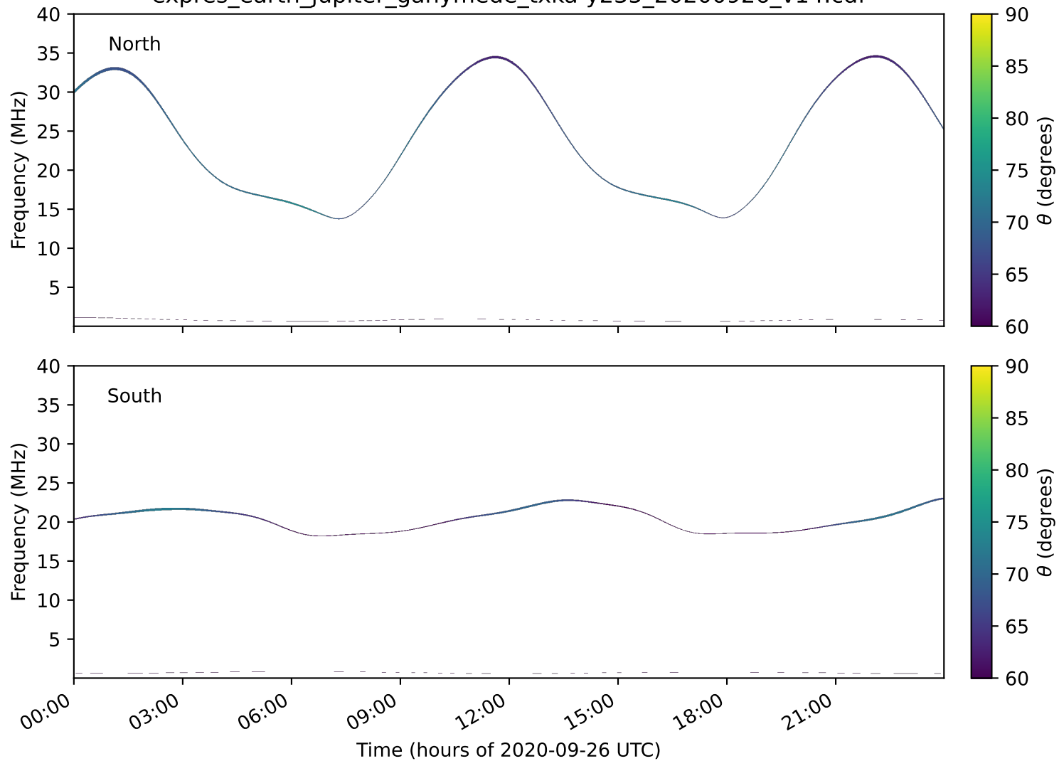
expres_earth_jupiter_ganymede_txka-y235_20200926_v14.cdf
