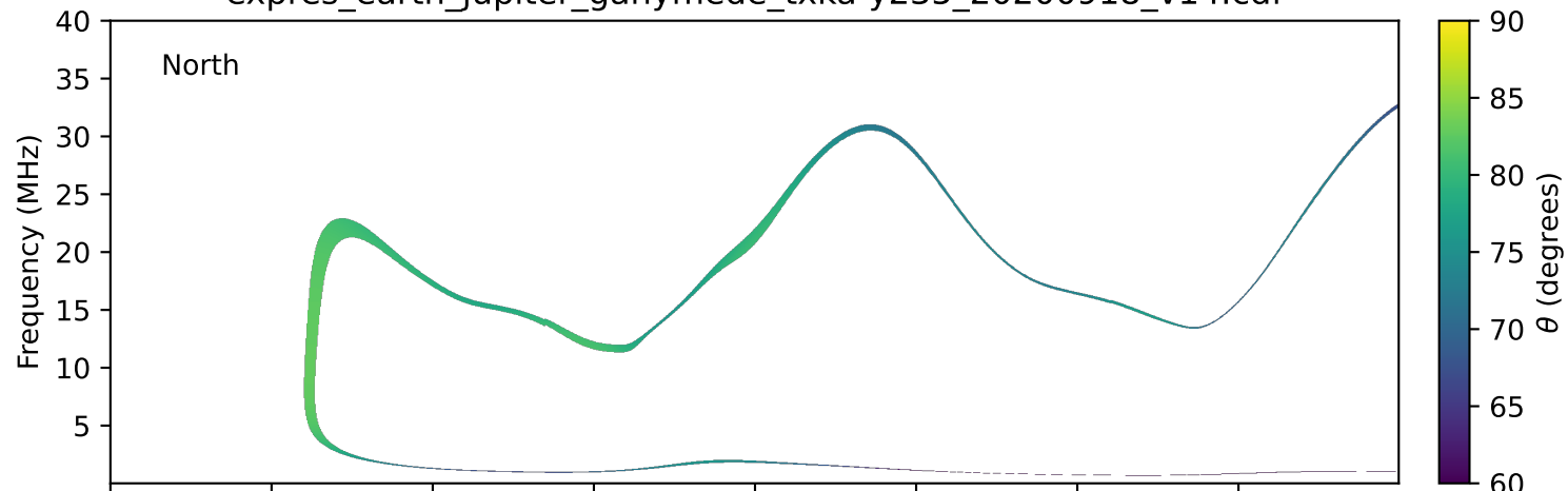
expres_earth_jupiter_ganymede_txka-y235_20200918_v14.cdf
