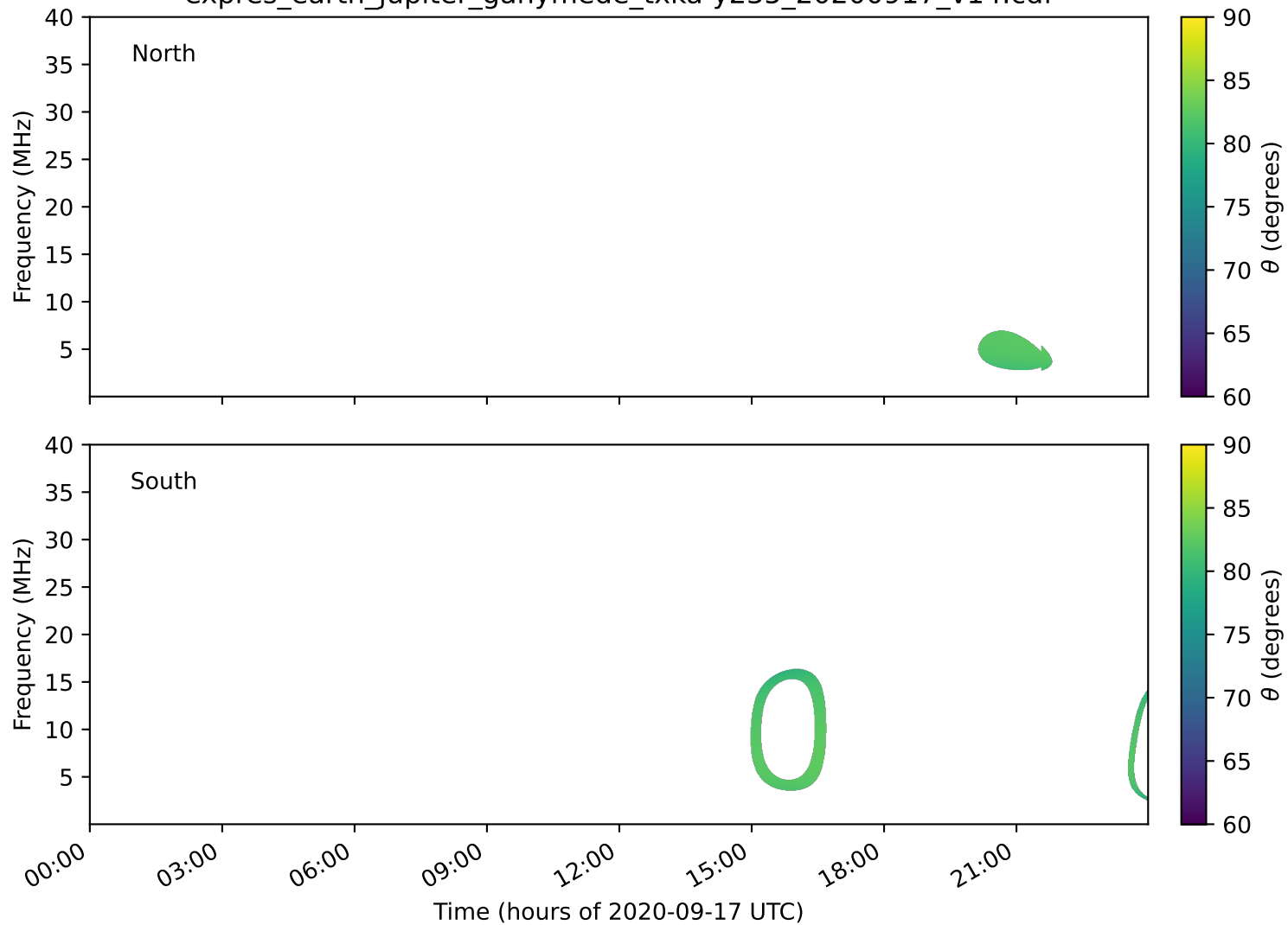
expres_earth_jupiter_ganymede_txka-y235_20200917_v14.cdf
