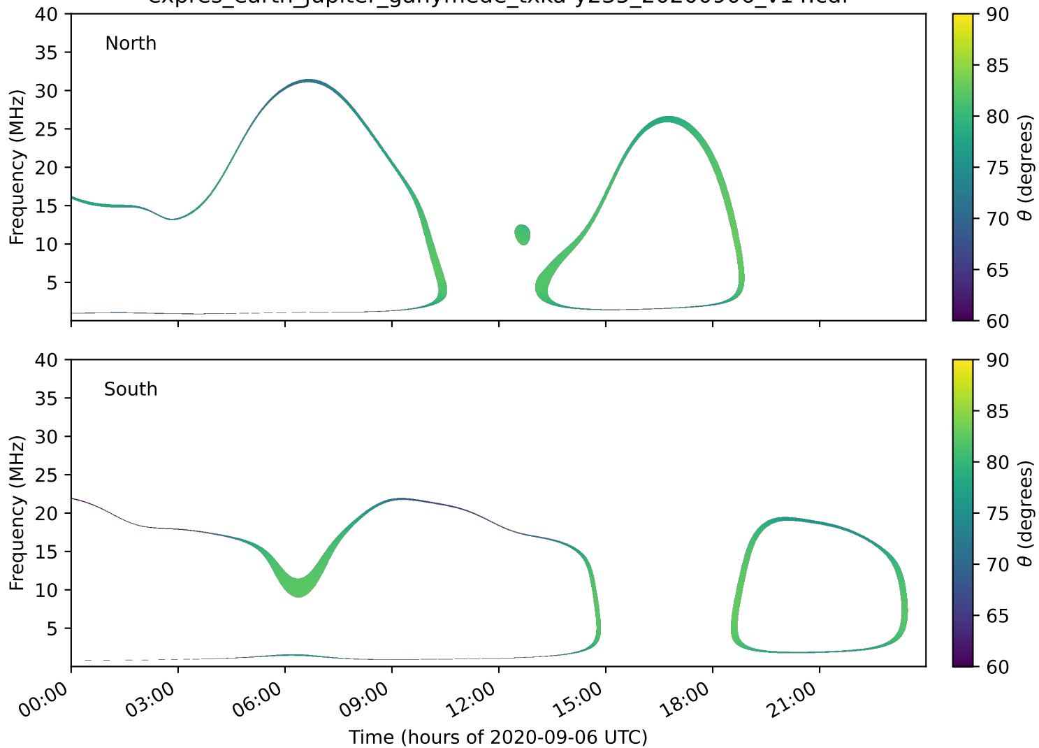
expres_earth_jupiter_ganymede_txka-y235_20200906_v14.cdf
