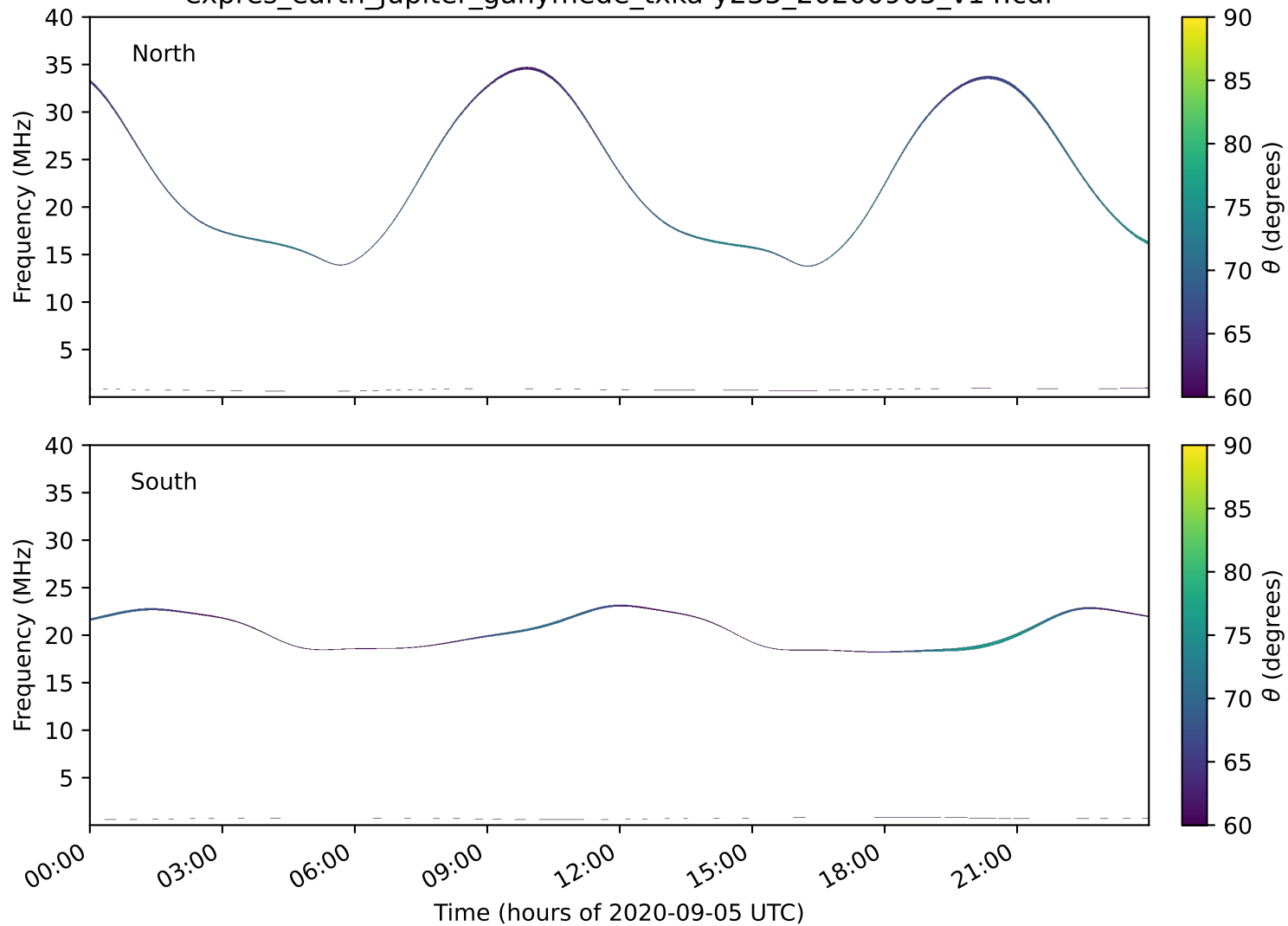
expres_earth_jupiter_ganymede_txka-y235_20200905_v14.cdf
