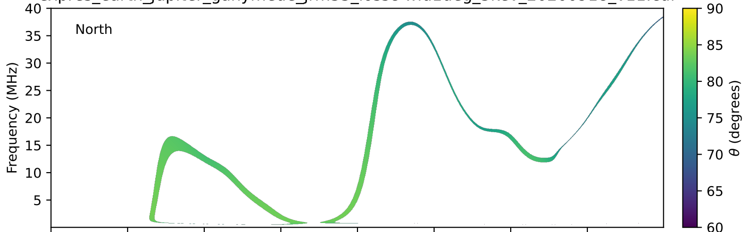
expres_earth_jupiter_ganymede_jrm33_lossc-wid1deg_3kev_20200918_v11.cdf
