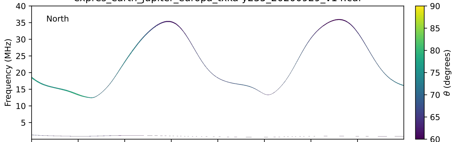
expres_earth_jupiter_europa_txka-y235_20200929_v14.cdf
