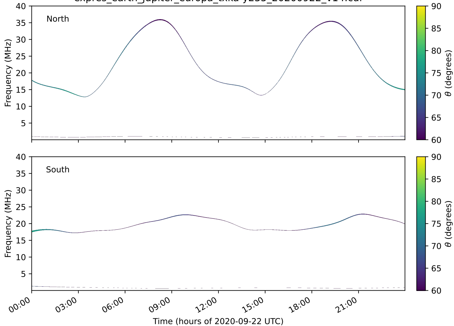
expres_earth_jupiter_europa_txka-y235_20200922_v14.cdf
