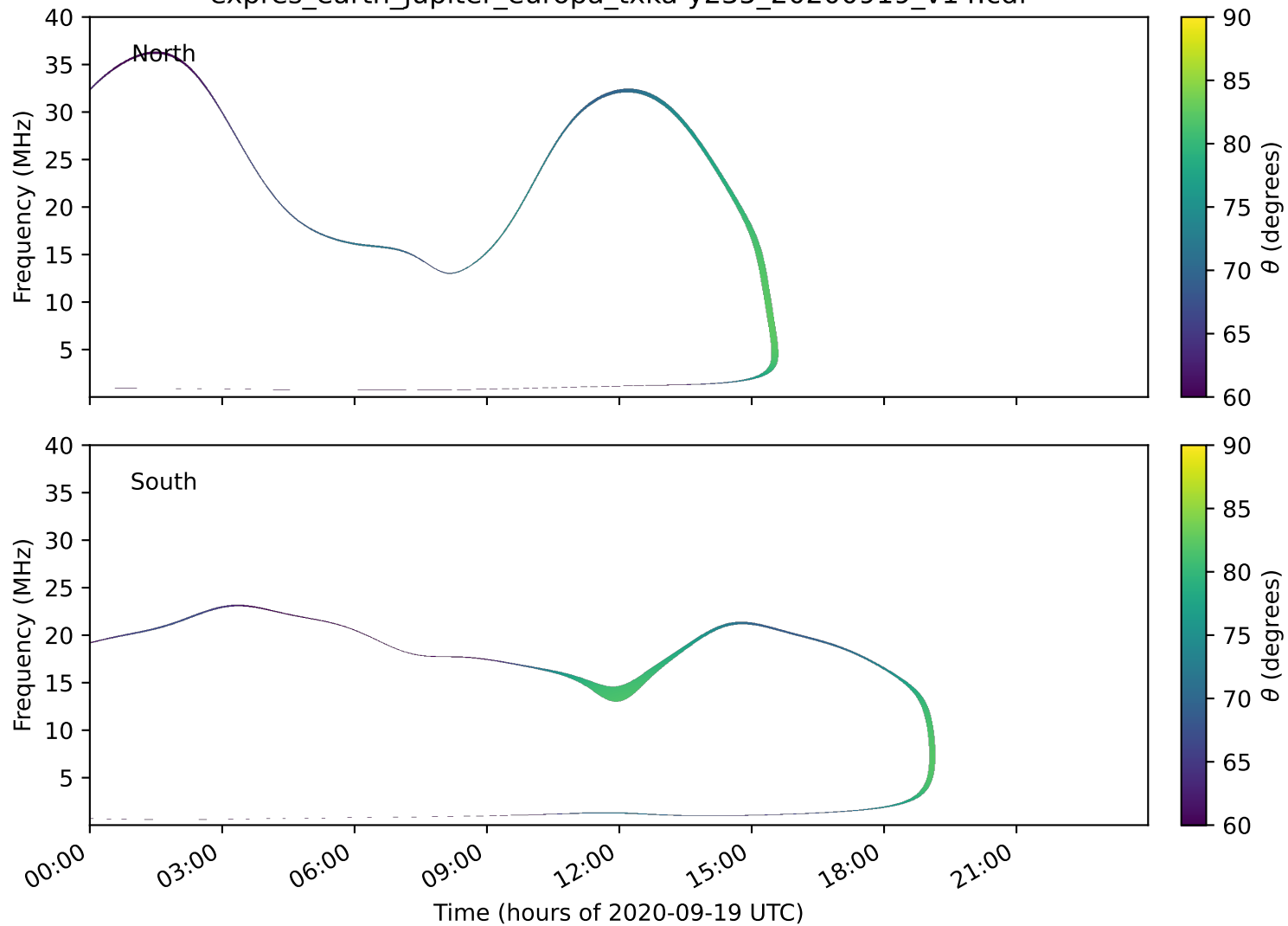
expres_earth_jupiter_europa_txka-y235_20200919_v14.cdf
