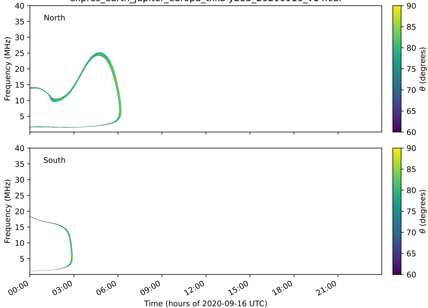
expres_earth_jupiter_europa_txka-y235_20200916_v14.cdf
