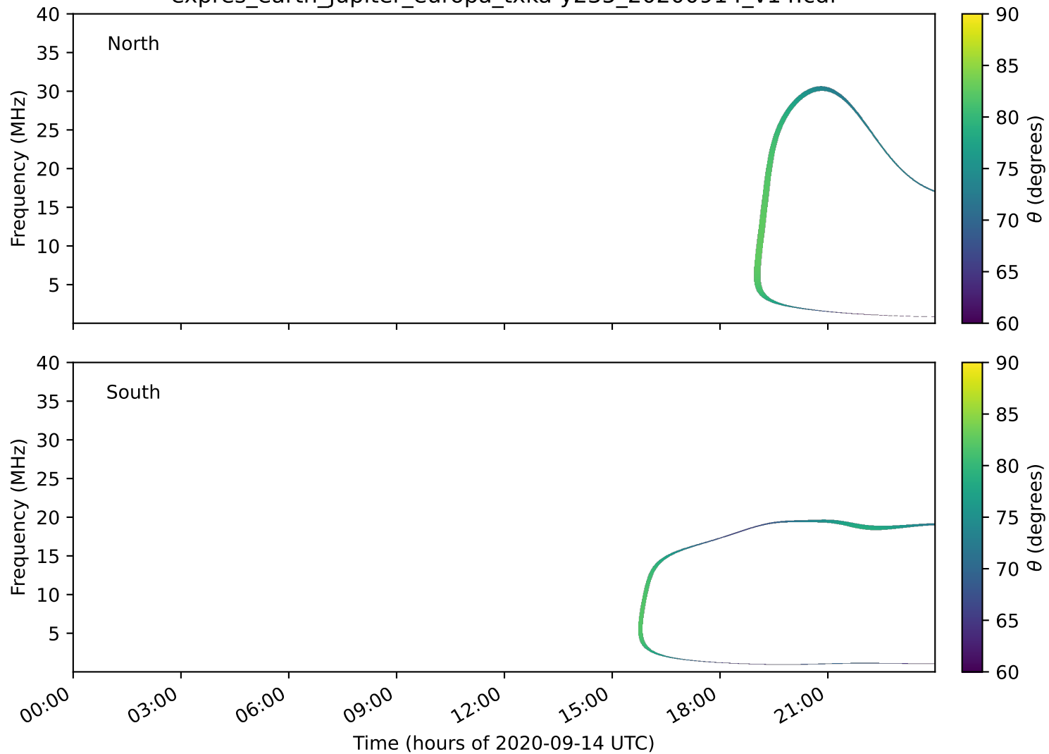
expres_earth_jupiter_europa_txka-y235_20200914_v14.cdf
