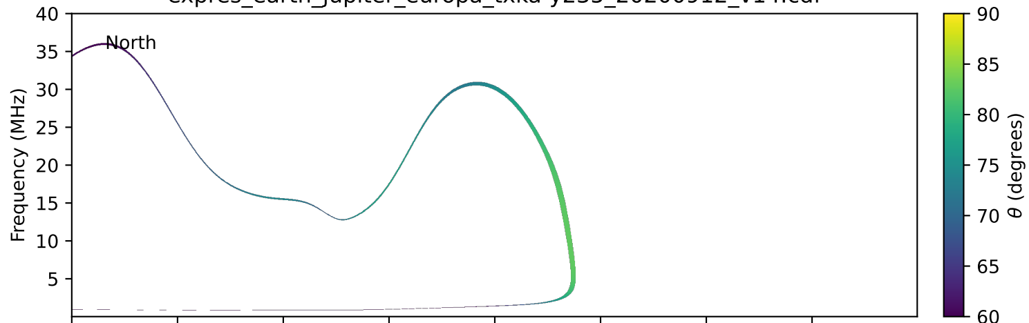
expres_earth_jupiter_europa_txka-y235_20200912_v14.cdf
