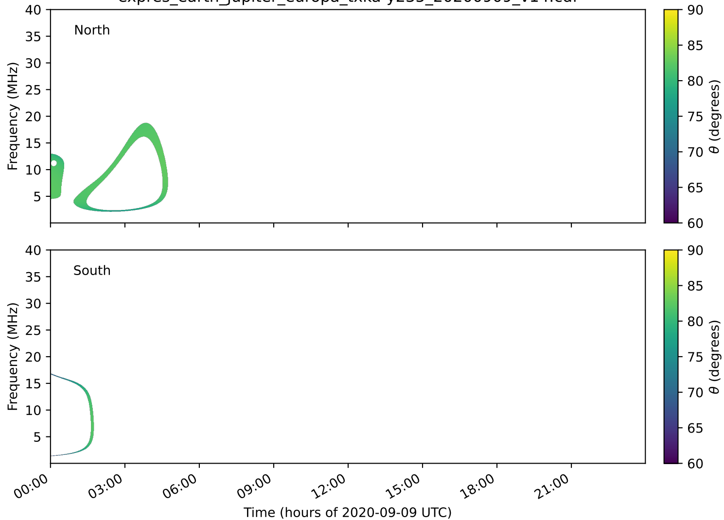
expres_earth_jupiter_europa_txka-y235_20200909_v14.cdf
