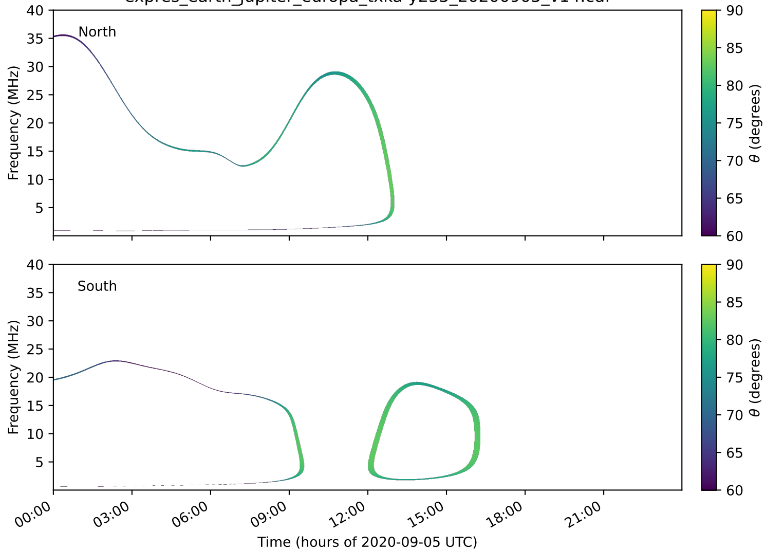
expres_earth_jupiter_europa_txka-y235_20200905_v14.cdf
