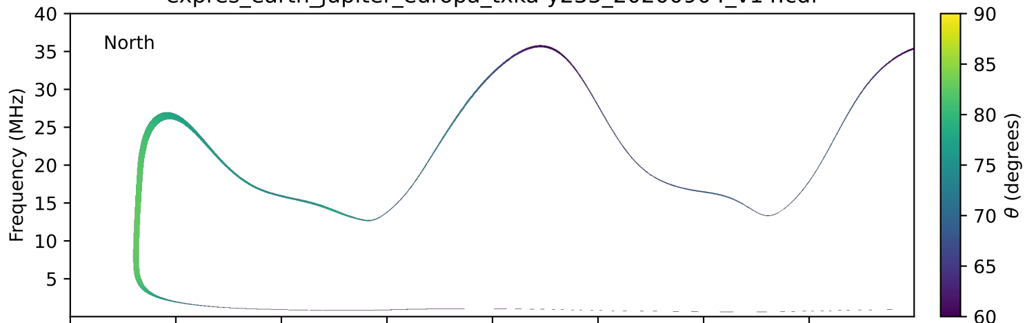
expres_earth_jupiter_europa_txka-y235_20200904_v14.cdf
