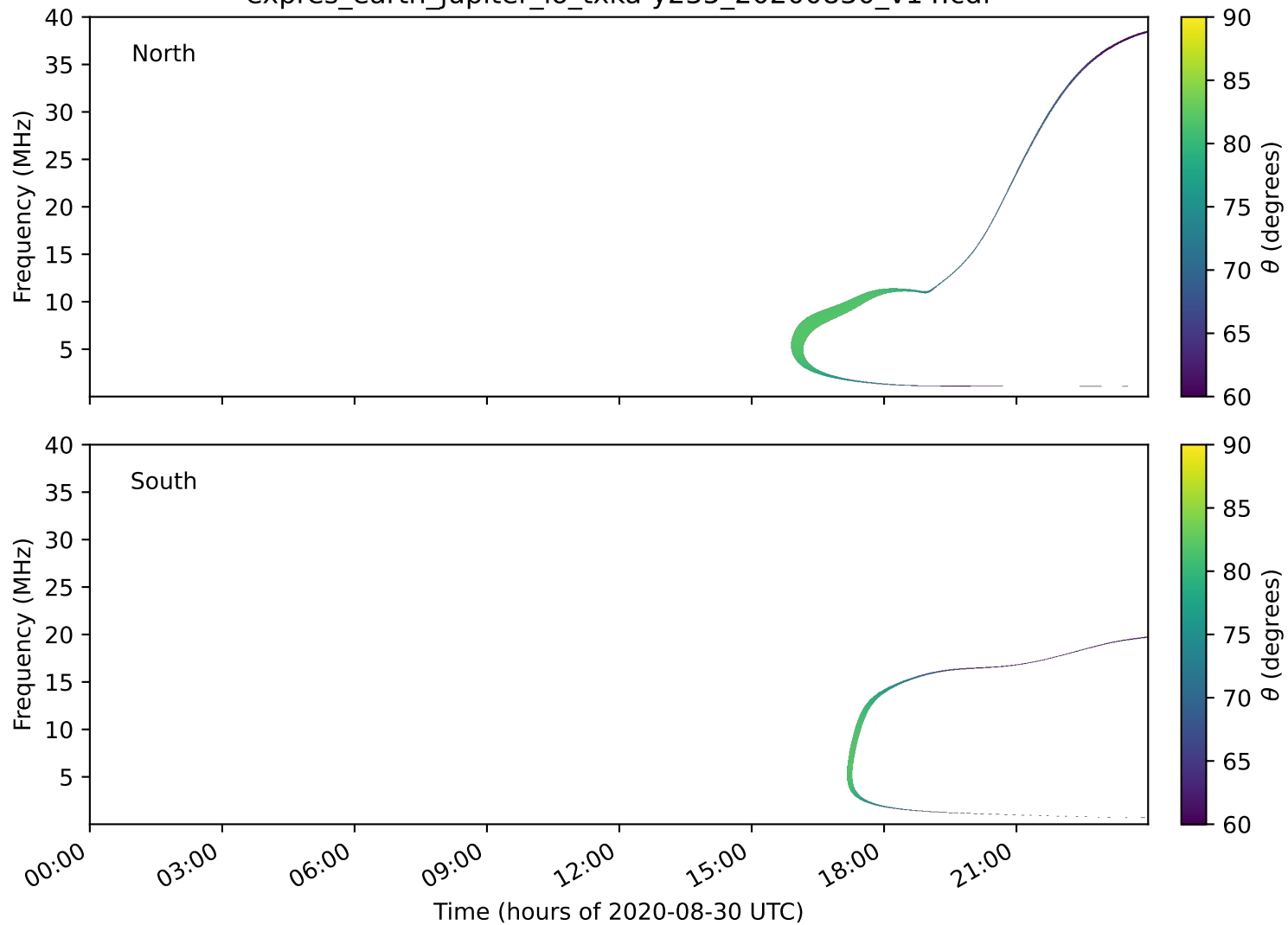
expres_earth_jupiter_io_txka-y235_20200830_v14.cdf
