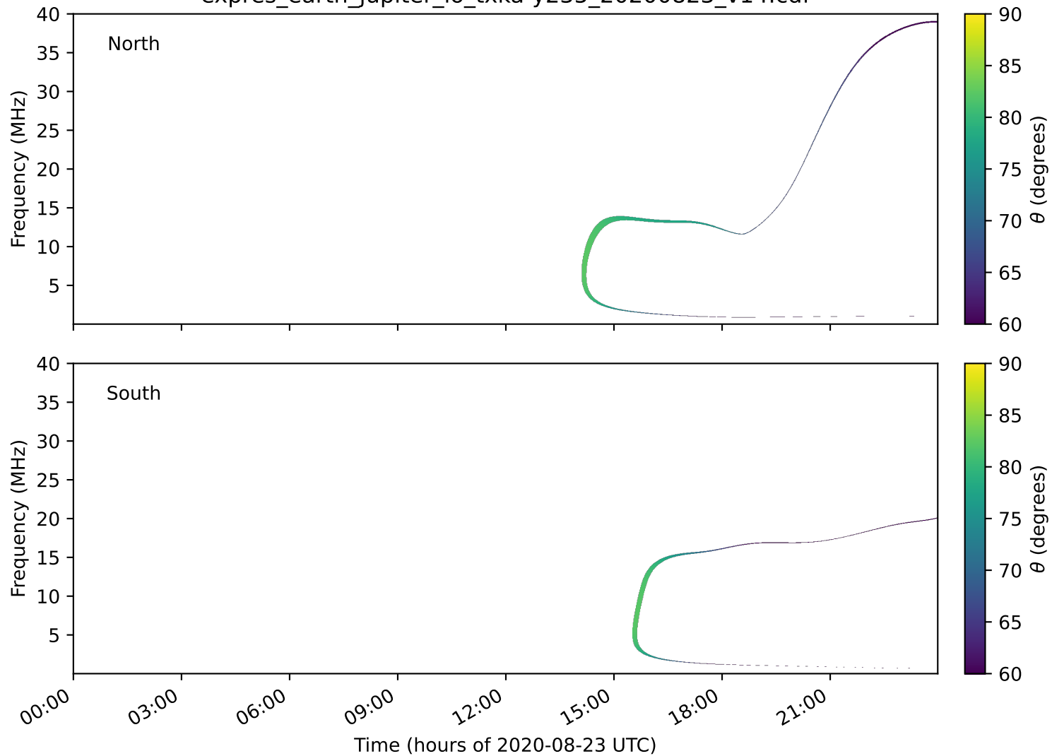
expres_earth_jupiter_io_txka-y235_20200823_v14.cdf
