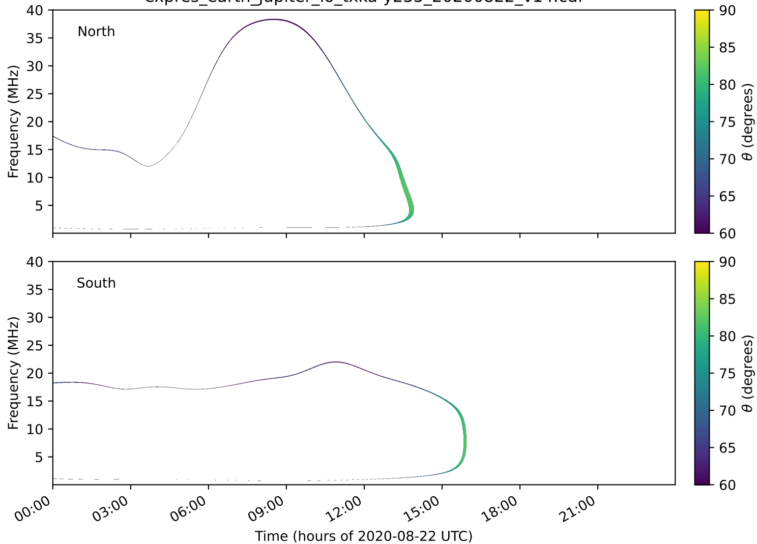
expres_earth_jupiter_io_txka-y235_20200822_v14.cdf
