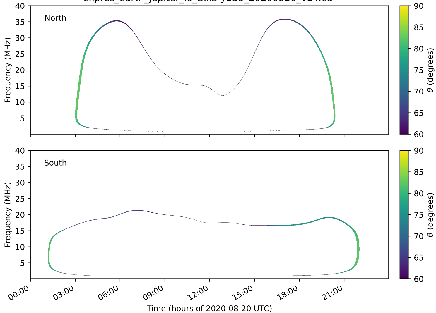
expres_earth_jupiter_io_txka-y235_20200820_v14.cdf
