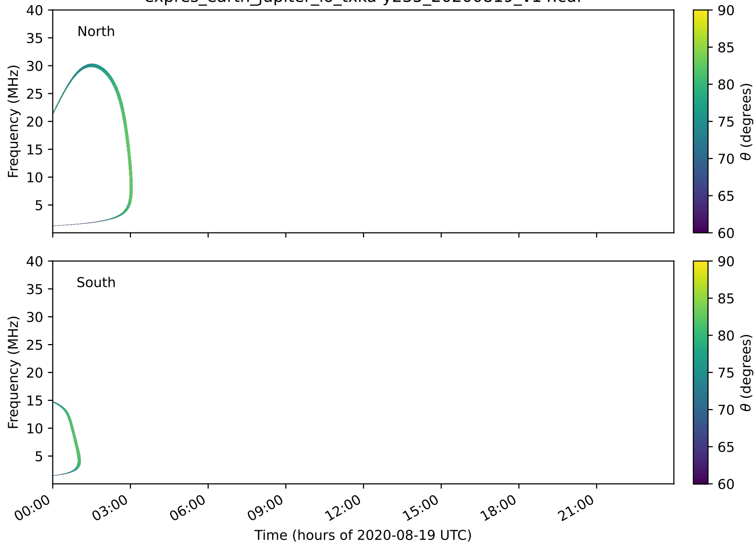
expres_earth_jupiter_io_txka-y235_20200819_v14.cdf
