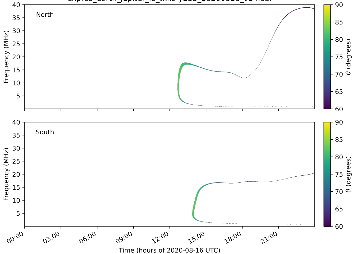
expres_earth_jupiter_io_txka-y235_20200816_v14.cdf
