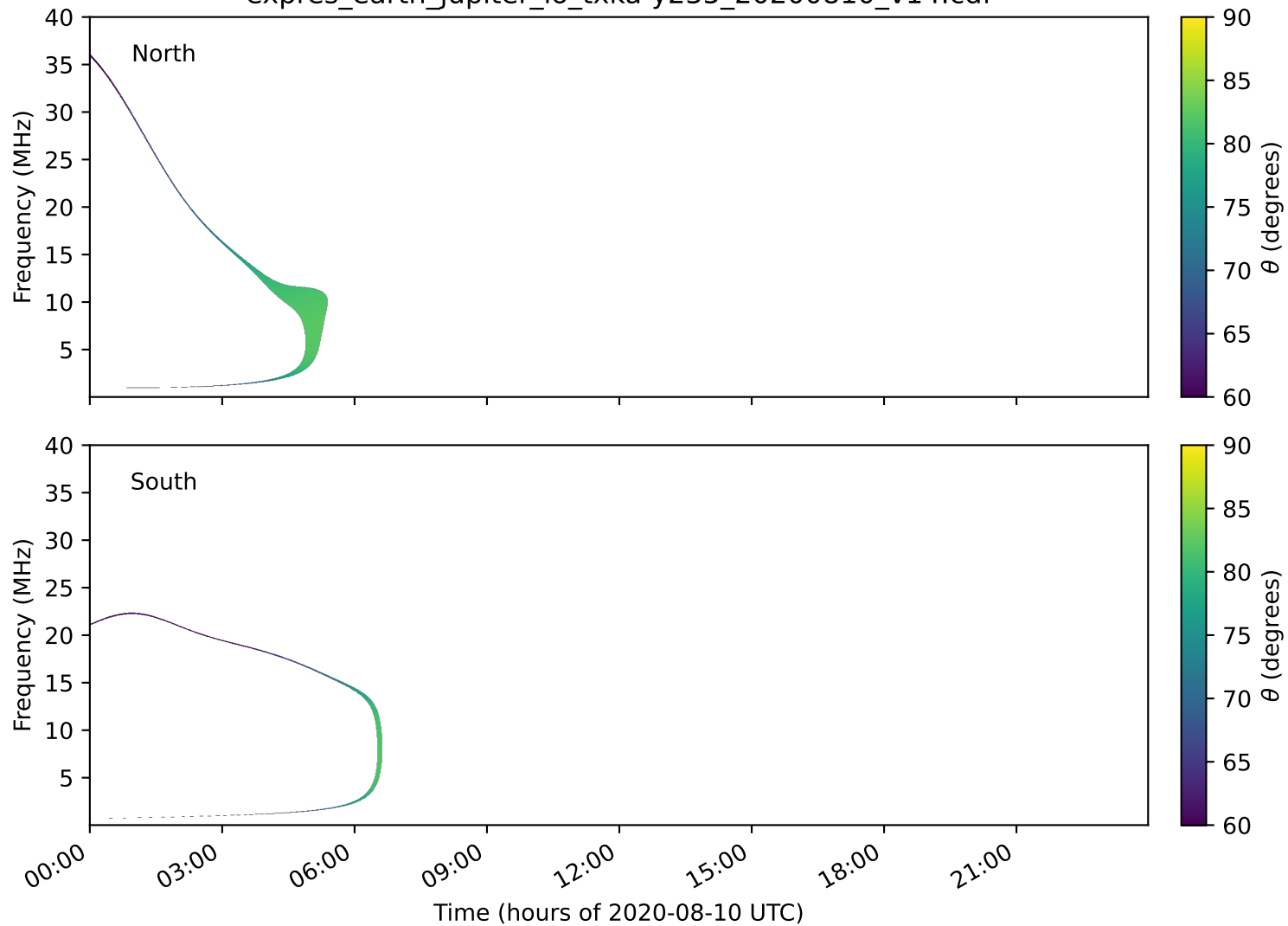
expres_earth_jupiter_io_txka-y235_20200810_v14.cdf
