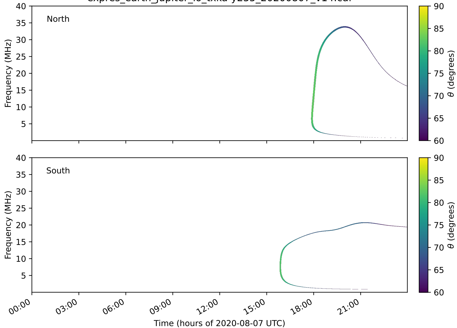
expres_earth_jupiter_io_txka-y235_20200807_v14.cdf
