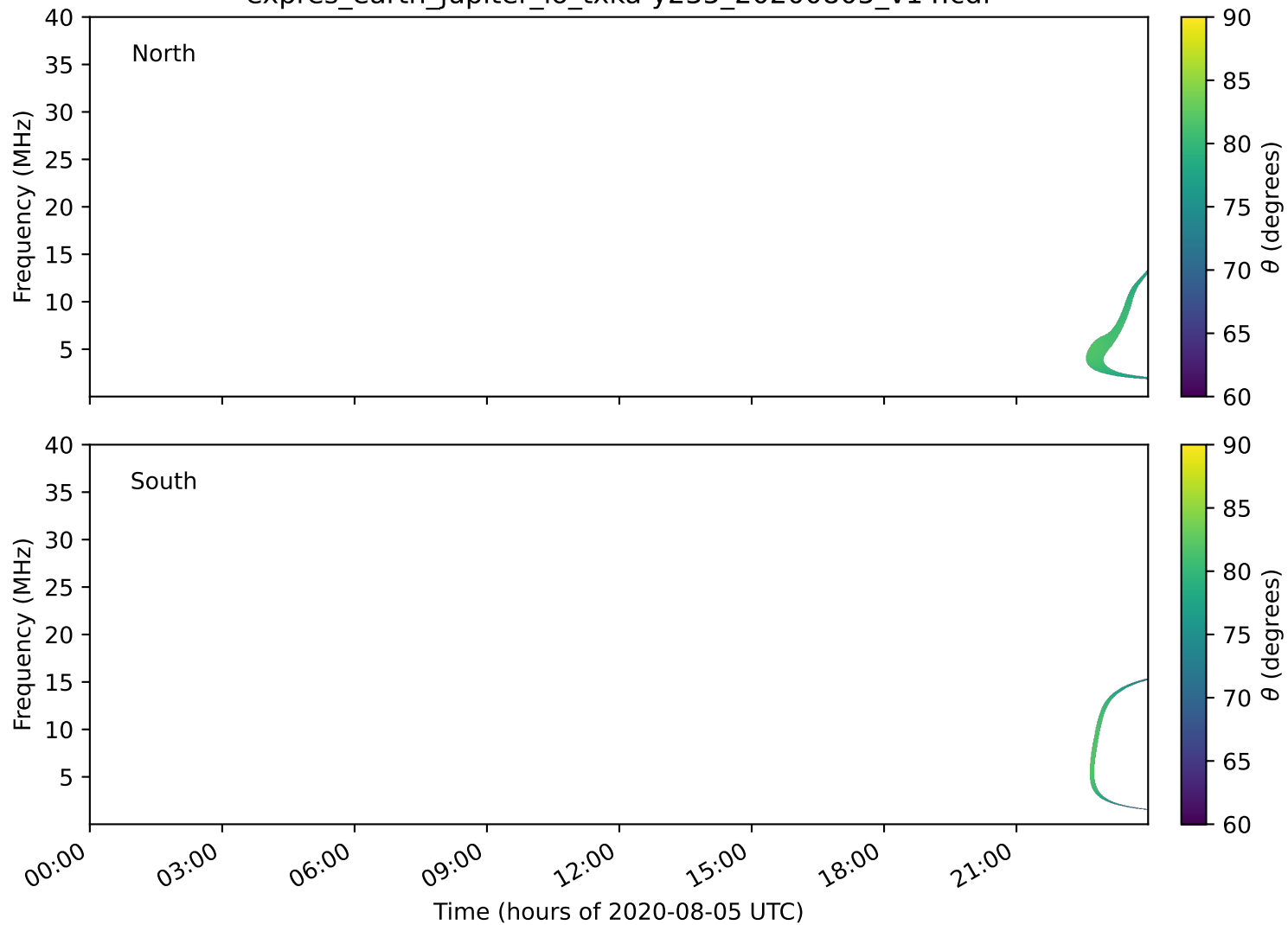
expres_earth_jupiter_io_txka-y235_20200805_v14.cdf
