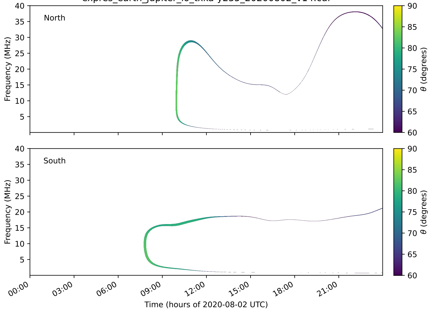
expres_earth_jupiter_io_txka-y235_20200802_v14.cdf
