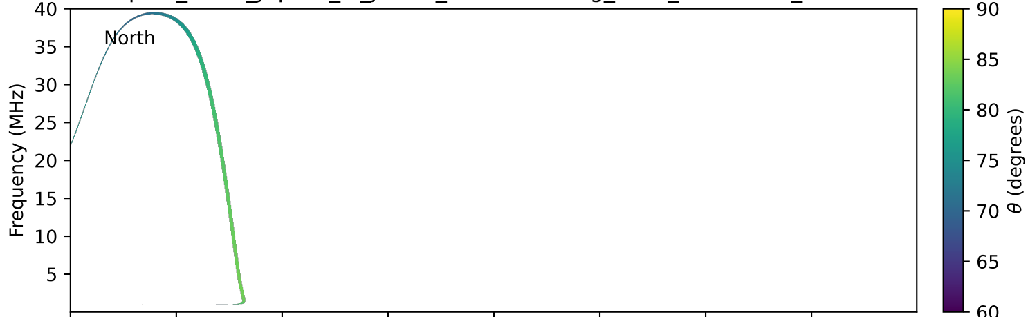
expres_earth_jupiter_io_jrm33_lossc-wid1deg_3kev_20200826_v11.cdf
