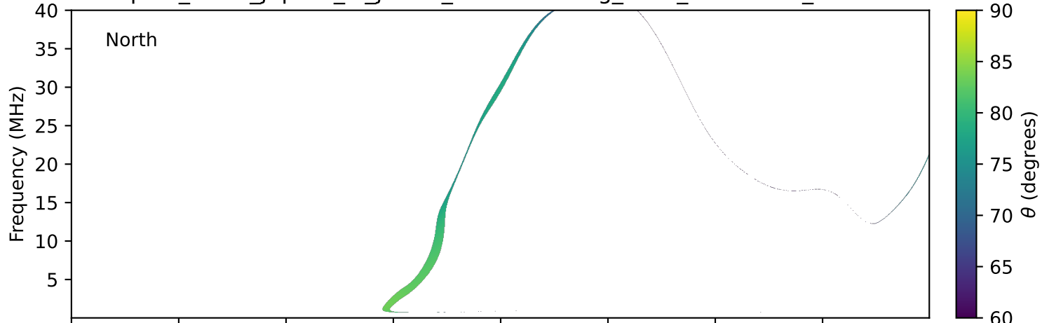
expres_earth_jupiter_io_jrm33_lossc-wid1deg_3kev_20200825_v11.cdf
