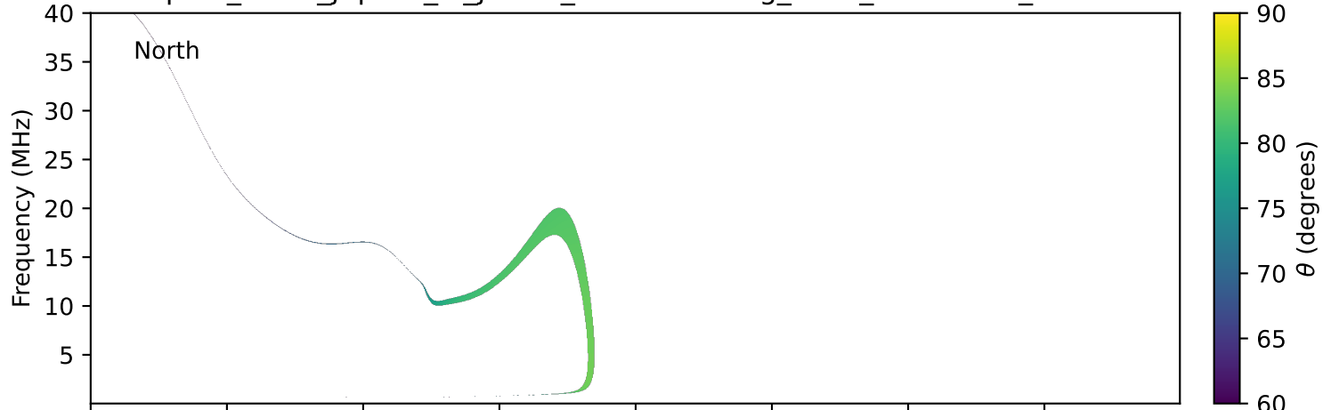
expres_earth_jupiter_io_jrm33_lossc-wid1deg_3kev_20200824_v11.cdf
